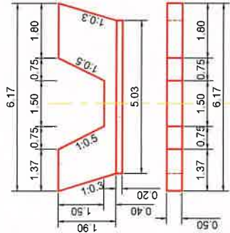
Band work No.8
