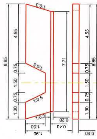
Band work No.3
