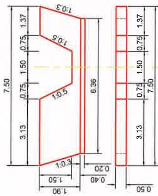
Band work No.7
