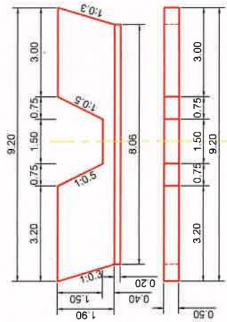
Band work No.6
